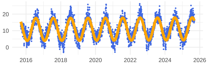
Temperature Model Fit (Last 10 years)
